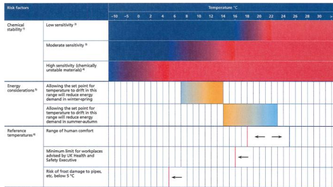
Figure C.1 – Relative risk of damage and deterioration due to temperature
